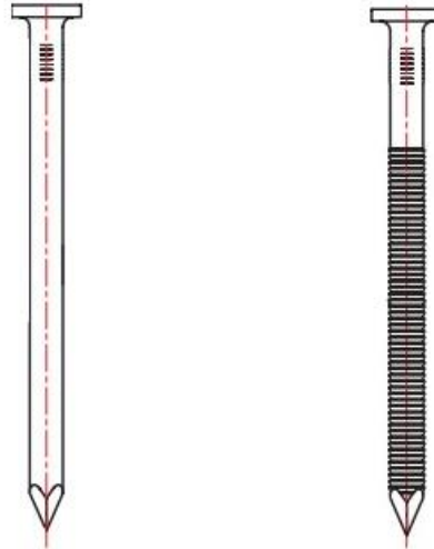
SMOOTH SHANK
